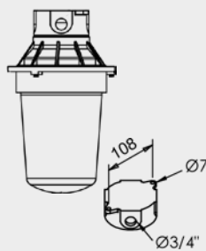
AY110/3P30 - Poste 30°
