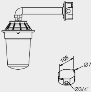
AY113 - Arandela 90°
